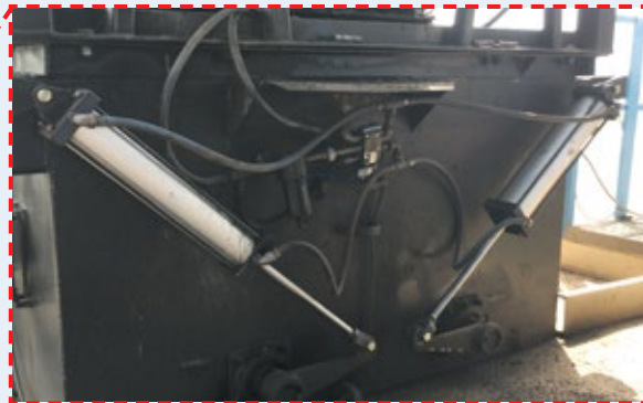
SHOWN: 4" x 16" batcher cylinders
